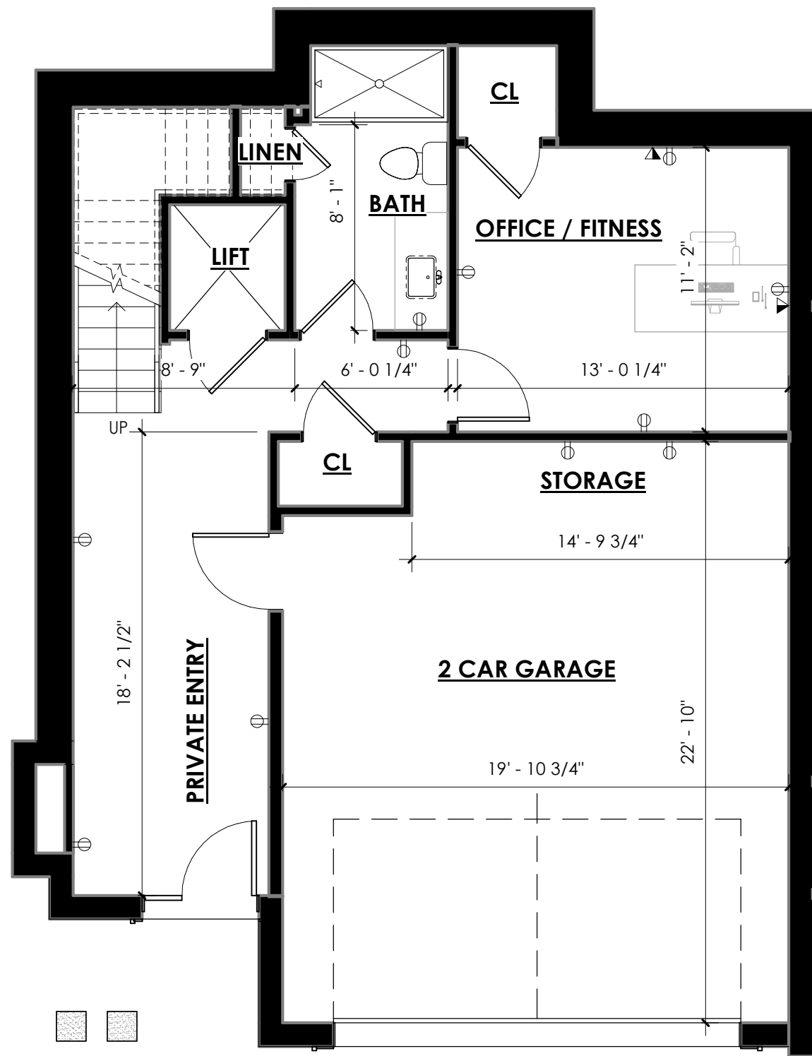
UNIT A PLAN - LEVEL 1 SCALE: 3/16" = 1'-0"
