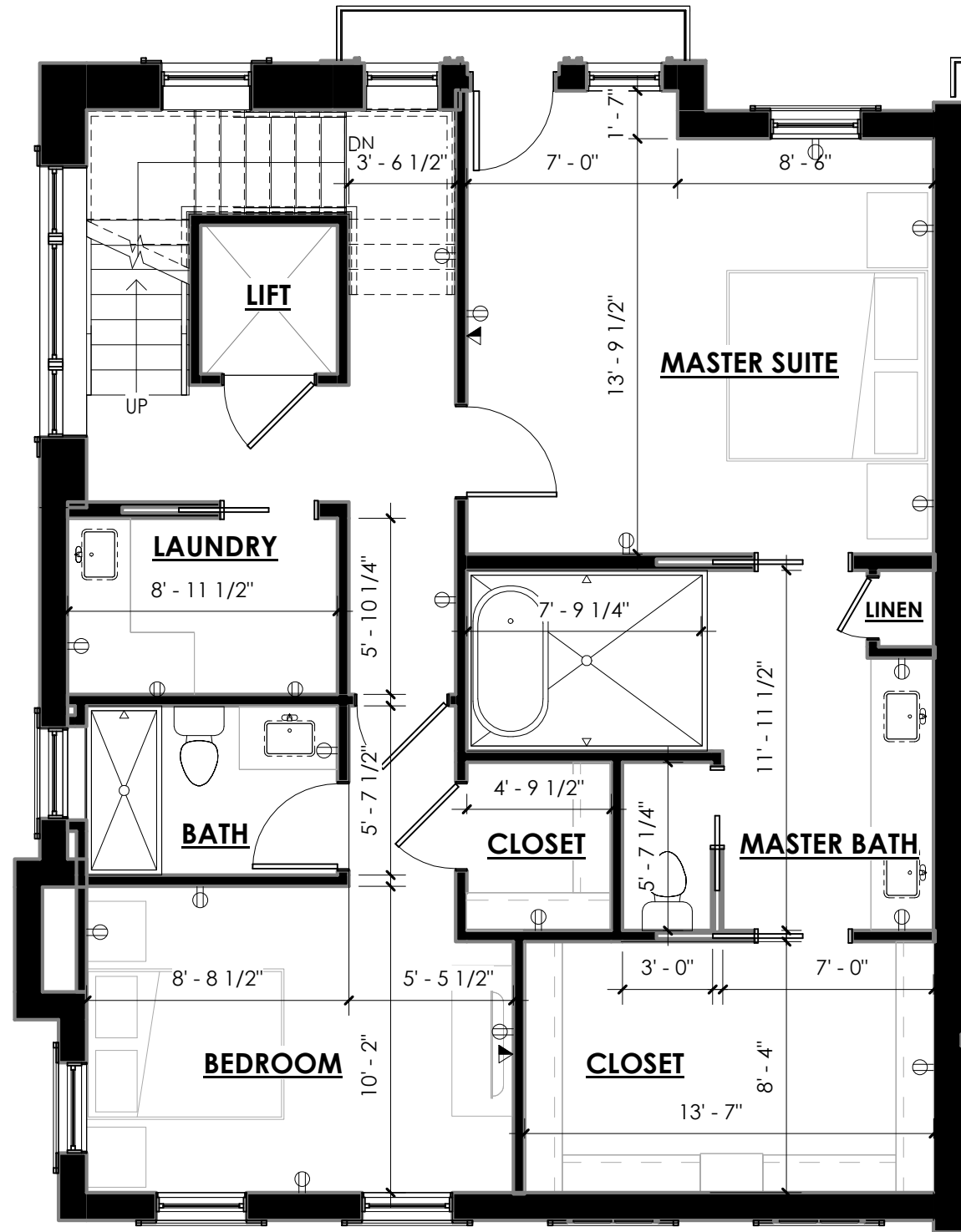
UNIT A PLAN - LEVEL 3
