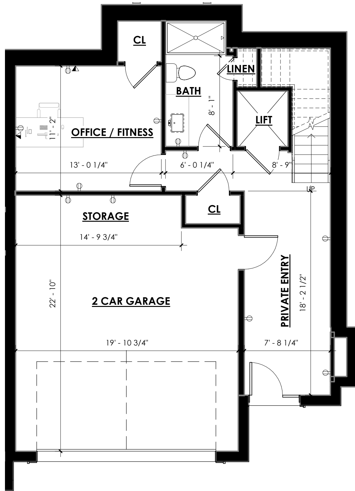
UNIT A PLAN (PRIME) - LEVEL 1 SCALE: 3/16" = 1'-0"
