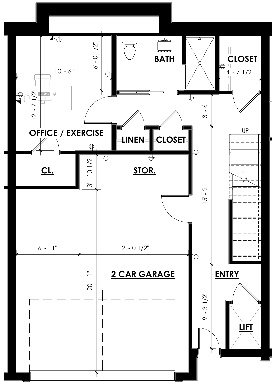
UNIT B PLAN - LEVEL 1
