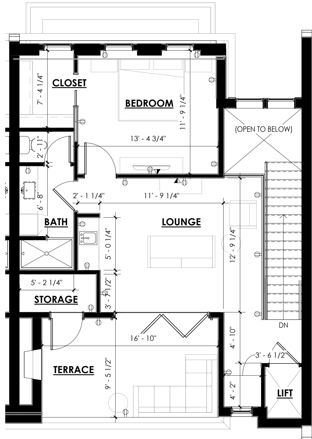
UNIT B PLAN - LEVEL 4
