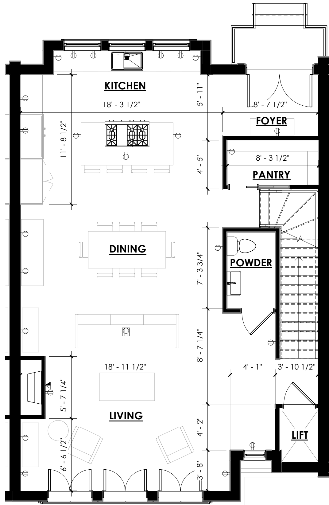
UNIT B PLAN - LEVEL 2
