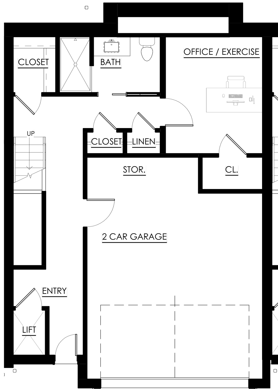
UNIT B PLAN (PRIME) -LEVEL 1 SCALE: 3/16" = 1'-0"
