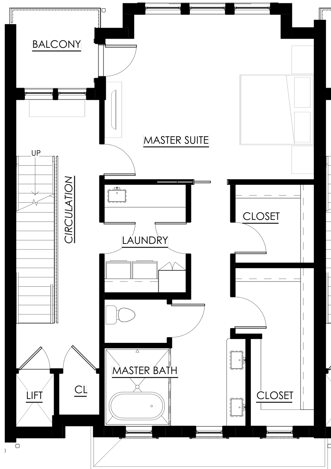
UNIT B PLAN (PRIME) -LEVEL 3 SCALE: 3/16" = 1'-0"
